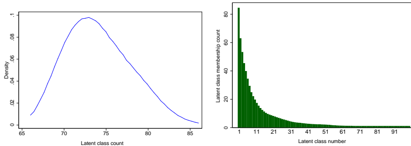
FIGURE 5. Density of the number of latent classes (left) and ordered average latent class membership counts (right).
