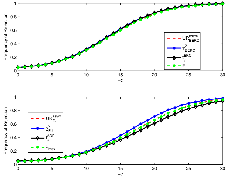
Figure 3: Local asymptotic power as a function of -c , R^2 = 0.25
