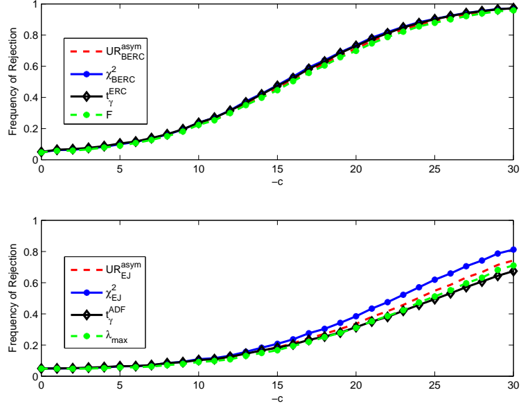
Figure 5: Local asymptotic power as a function of c , R^2 = 0.35 , K - 1 = 3
