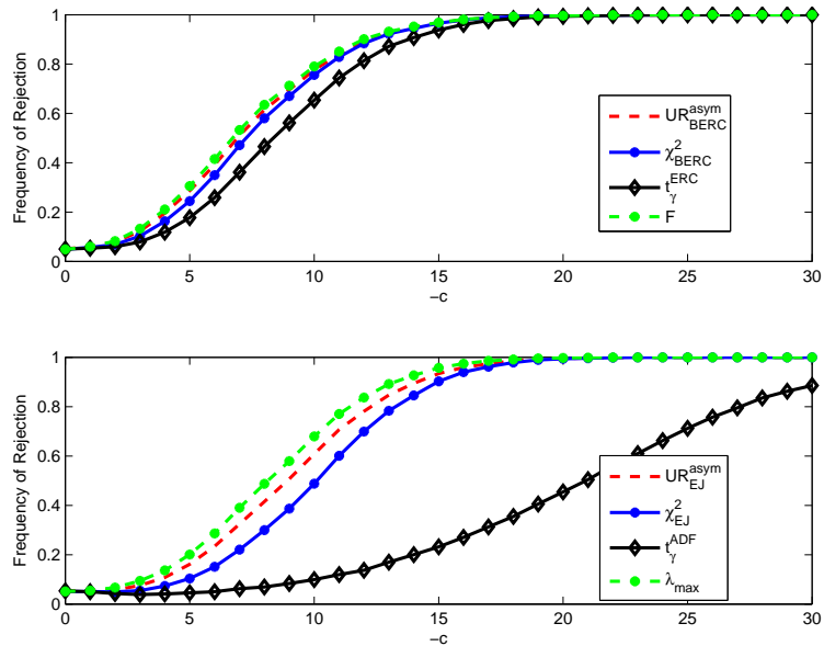
Figure 4: Local asymptotic power as a function of -c , R^2 = 0.7
