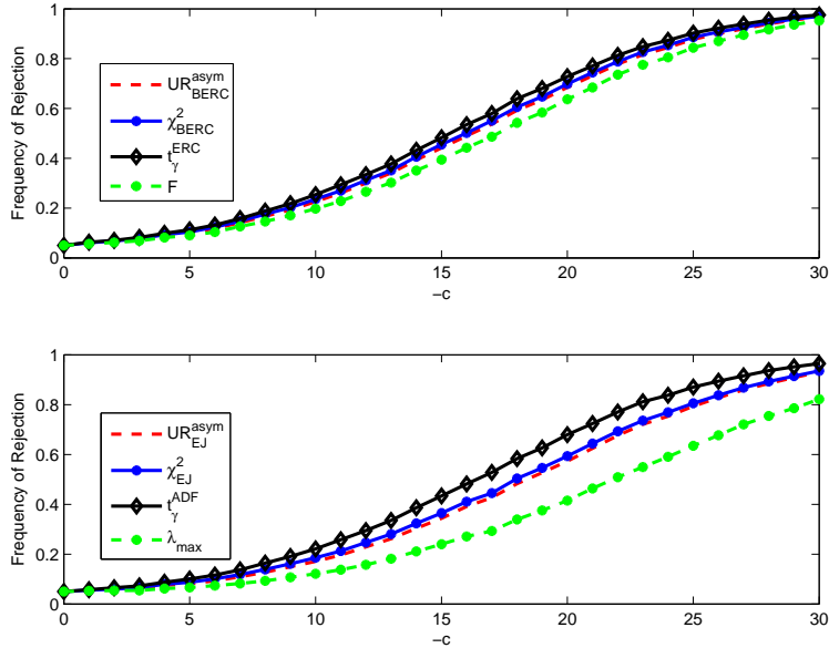
Figure 2: Local asymptotic power as a function of -c , R^2 = 0
