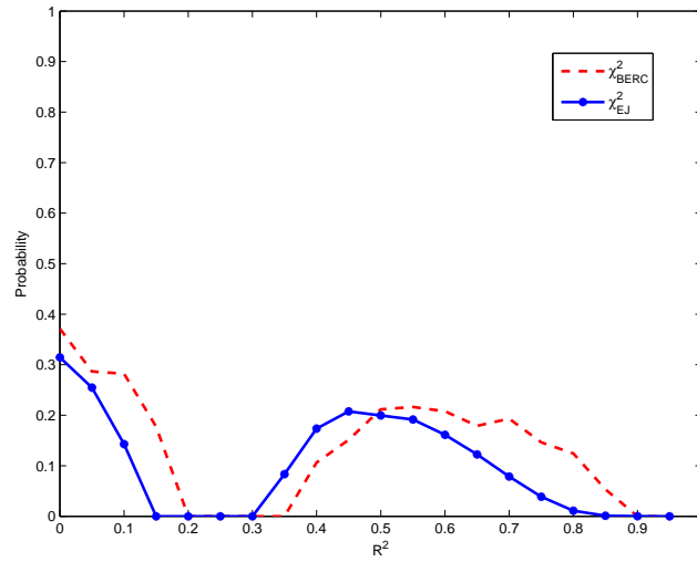
Figure 6: Cutoff probability q
